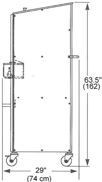
SIDE VIEW Outside Dimensions
